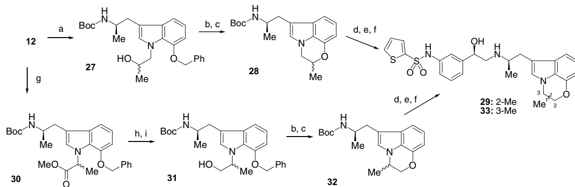
Scheme 7. Reagents: (a) propylene oxide, t -BuOK, THF; (b) 10% Pd–C, H 2 , EtOH; (c) DEAD, Ph 3 P, THF; (d) 4M HCl–EtOAc; (e) 4 , KI, i -Pr 2 NEt, MeCN; (f) 4M HCl–EtOAc, EtOH; (g) methyl 2-bromopropionate, NaH, DMF; (h) 1M NaOHaq, MeOH; (i) BH 3 –THF complex, THF.
