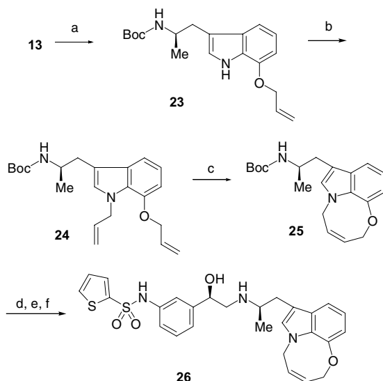
Scheme 6. Reagents: (a) allyl iodide, K 2 CO 3 , acetone; (b) allyl bromide, NaH, DMF; (c) Cl 2 (PCy 3 ) 2 Ru=CHPh, CH 2 Cl 2 ; (d) 4M HCl-EtOAc; (e) 4 , KI, i -Pr 2 NEt, MeCN; (f) 4M HCl-EtOAc, EtOH.
