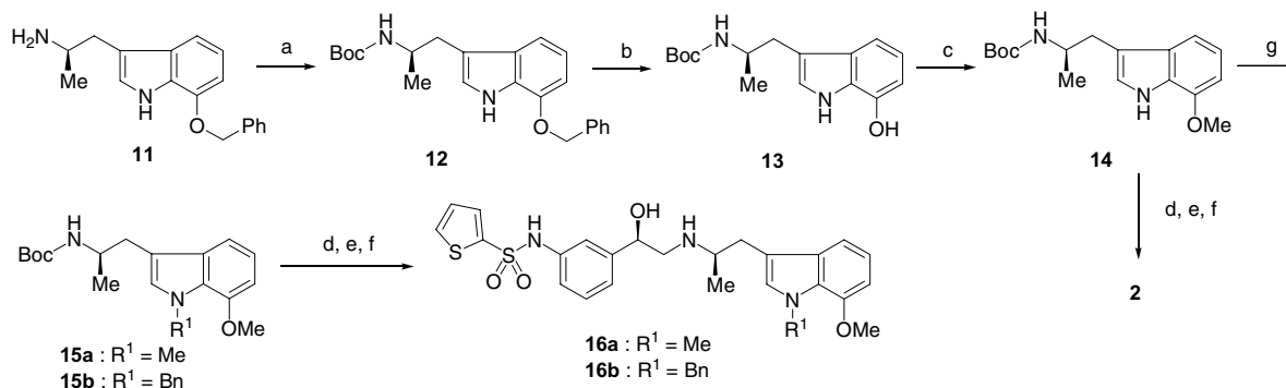
Scheme 3. Reagents: (a) (Boc) 2 O, EtOAc; (b) 5% Pd–C, MeOH; (c) MeI, K 2 CO 3 , acetone; (d) 4M HCl–EtOAc; (e) 4 , KI, i -Pr 2 NEt, MeCN; (f) 4M HCl–EtOAc, EtOH; (g) MeI or BnBr, NaH, DMF.
