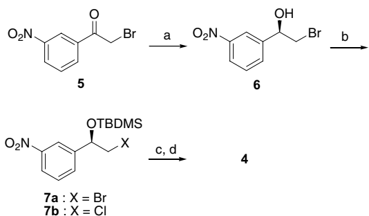
Scheme 1. Reagents: (a) ( R )-2-methyl-CBS-oxazaborolidine, \text{BH}_3 –THF complex, THF; (b) TBDMSCl, KBr, imidazole, DMF; (c) 5% Pt/C, \text{H}_2 , EtOAc; (d) 2-thiophenylsulfonyl chloride, pyridine, \text{CH}_2\text{Cl}_2 .
